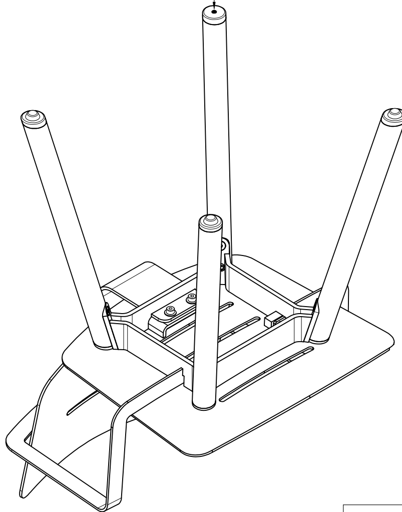
ISO VIEW
