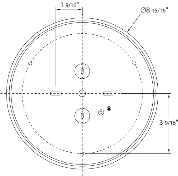
Back Plate Dimensions
