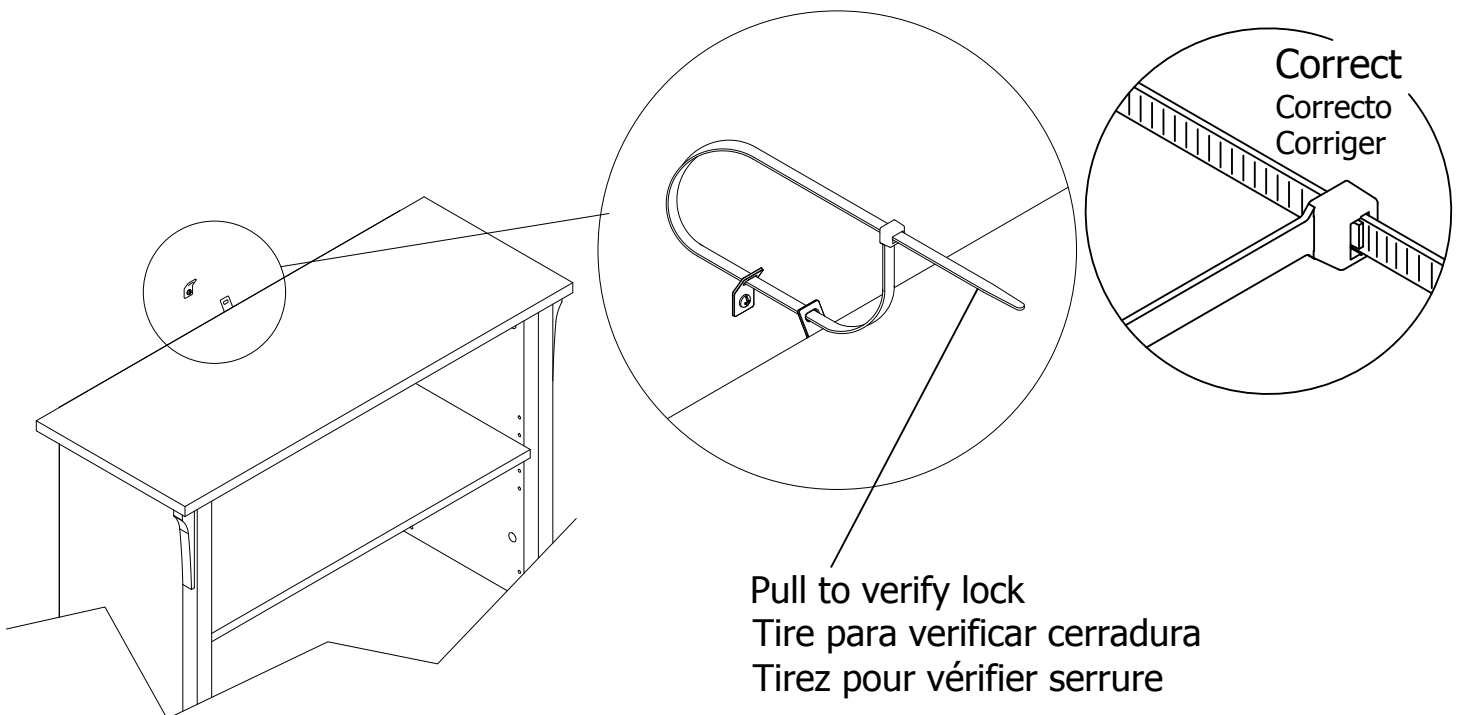
Nylon Cable Tie
