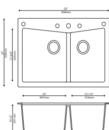
KGD-430B 33" x 22" x 9 1/2" Min Cabinet Size: 36" Drain Model #: BST-2 & ST-2
