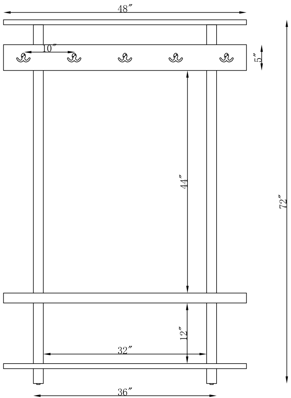
FRONT VIEW
