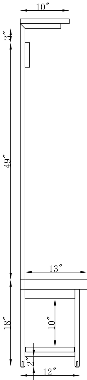
SIDE VIEW
