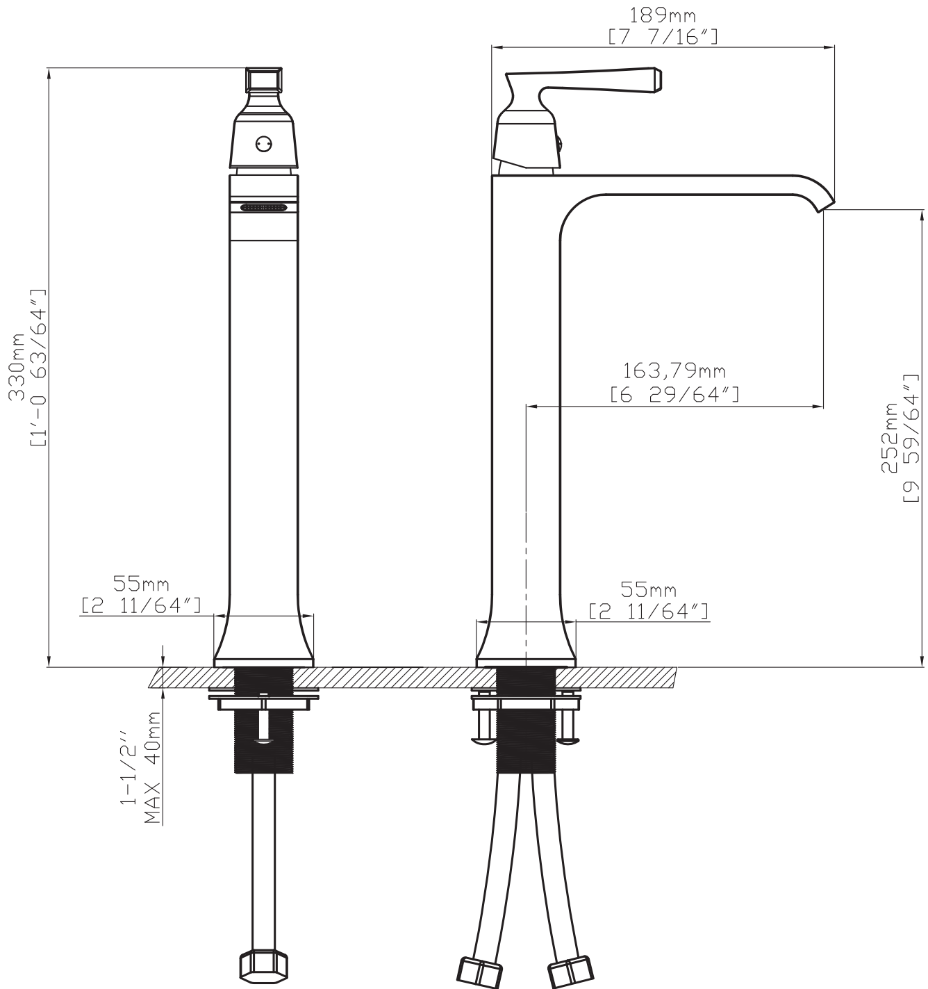
Front View
