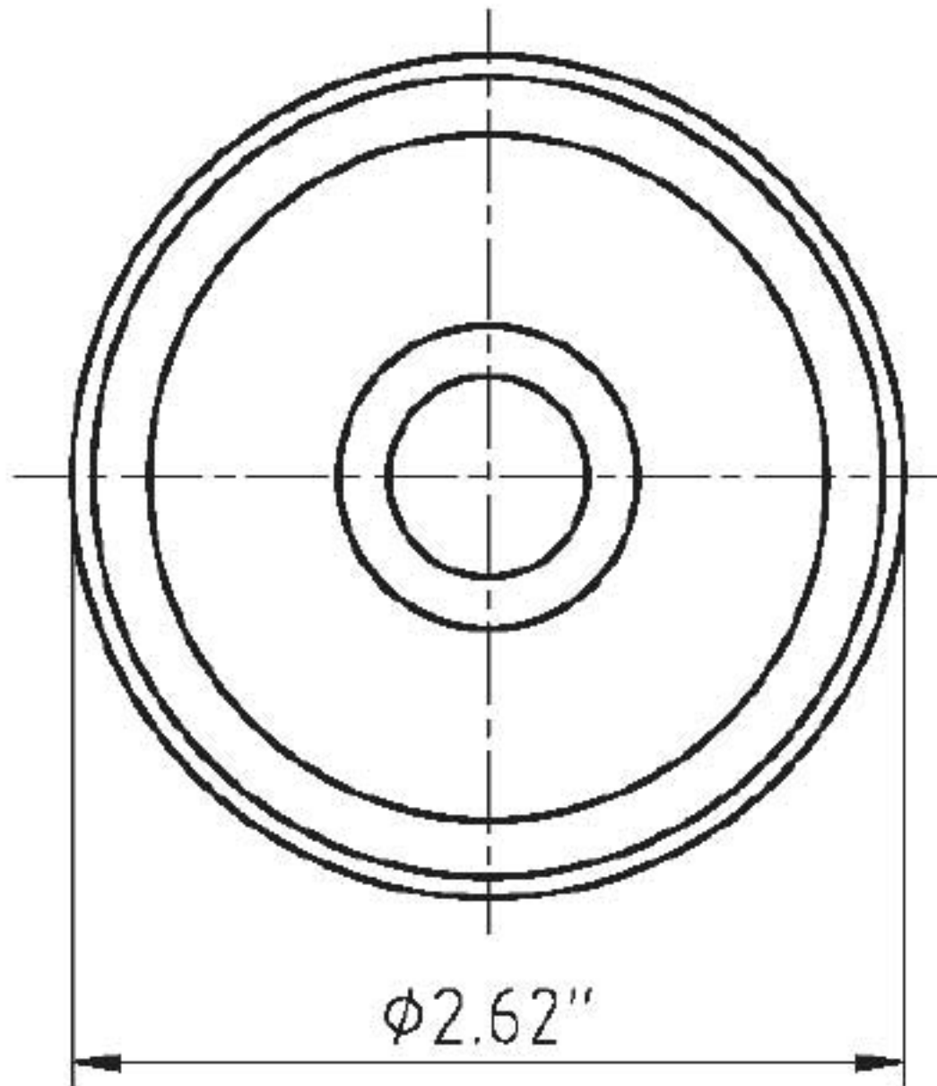
Front View
