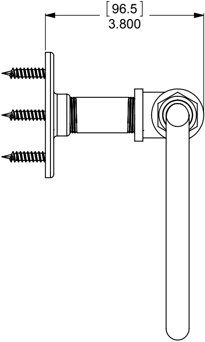
DETAIL T SCALE 2 : 3
