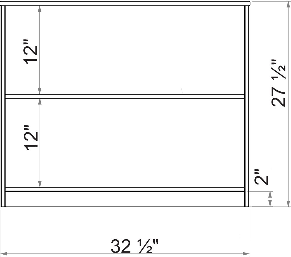
Frontal View
