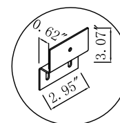
Metal bracket
