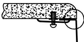
Flushed/Zero Reveal
