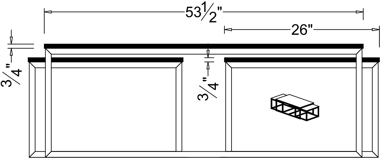
FRONT VIEW
