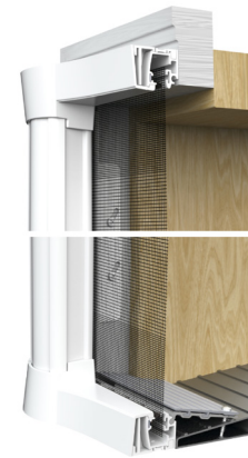
Surface/Face Mounting on a Traditional Hinged Door
