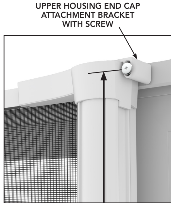
78 1/2" TO SCREW CENTERS
