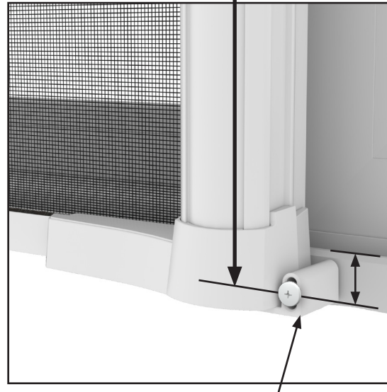
LOWER HOUSING END CAP ATTACHMENT BRACKET WITH SCREW
