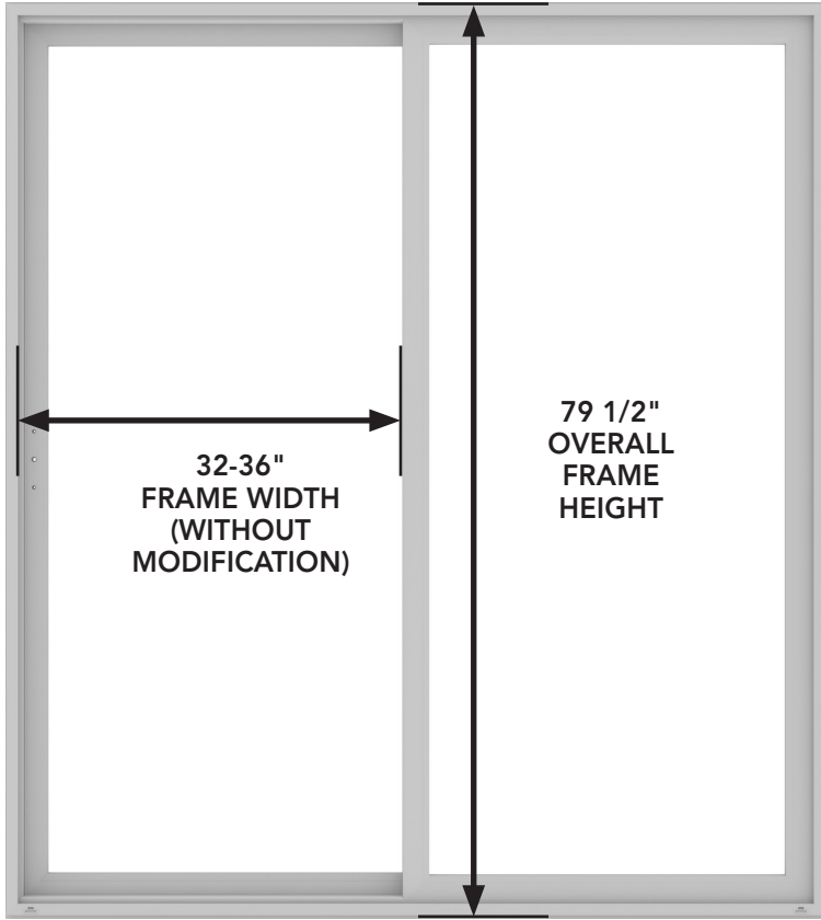
EXTERIOR VIEW
