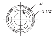
Mounting Ring Dimensions
