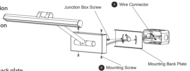
Fig.2 MOUNT ON JUNCTION BOX
