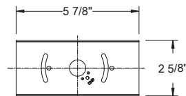
Mounting Ring Dimensions
