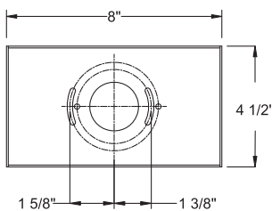
Conversion Plate Dimensions
