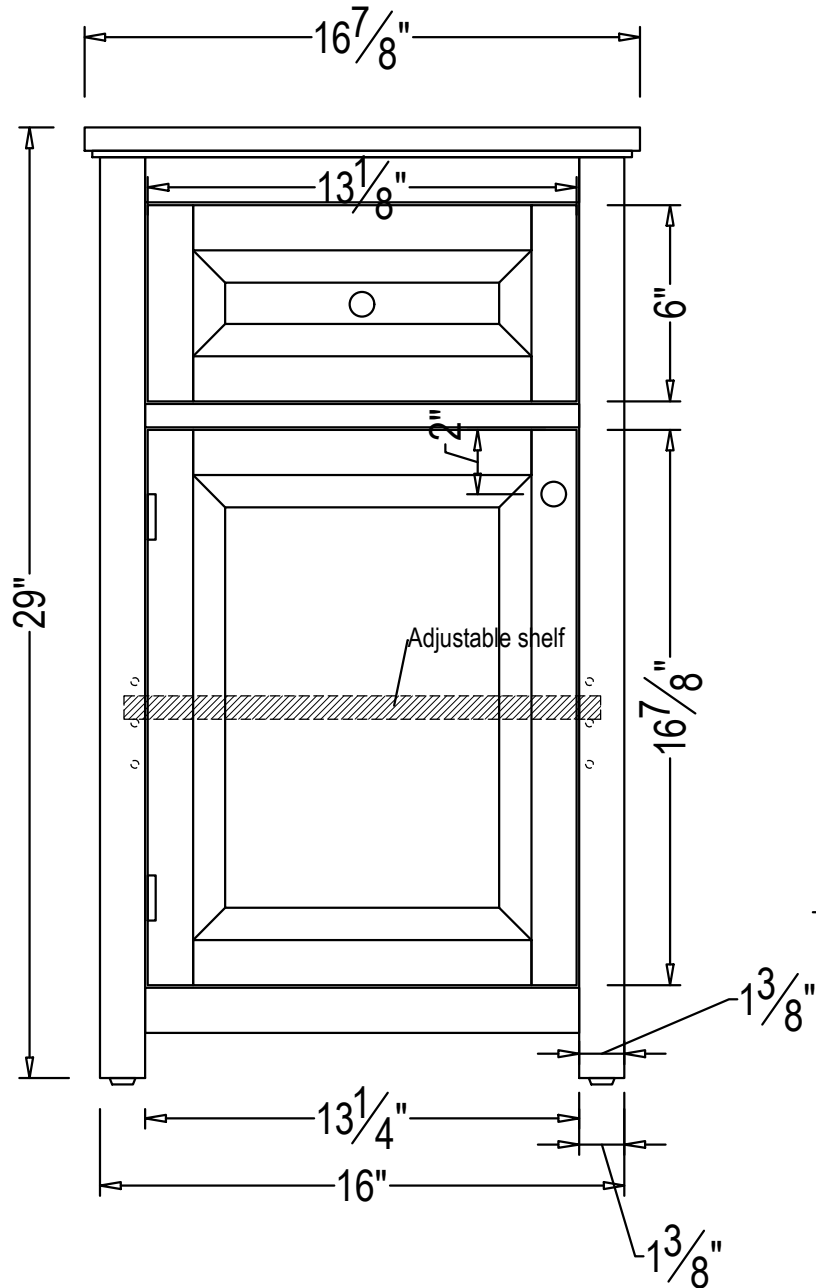
STORAGE BASE
