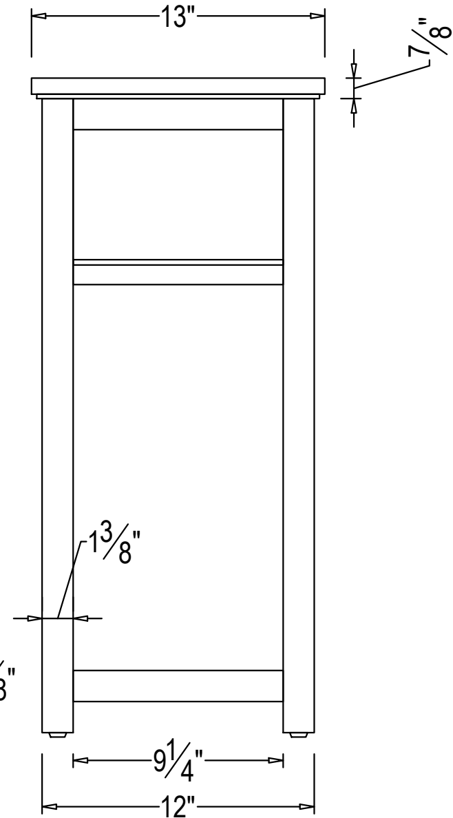
SIDE VIEW
