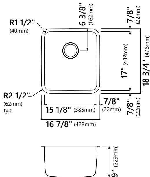
KA1US17B 16\ 7/8'' \times 18\ 3/4'' \times 9'' Min Cabinet Size: 21"
