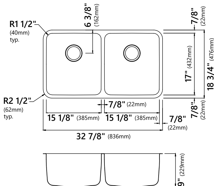
KA1UD33B 32\ 7/8'' \times 18\ 3/4'' \times 9'' Min Cabinet Size: 36"
