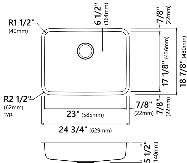
KA1AS25B 24\ 3/4'' \times 18\ 7/8'' \times 5\ 1/2'' Min Cabinet Size: 30"
