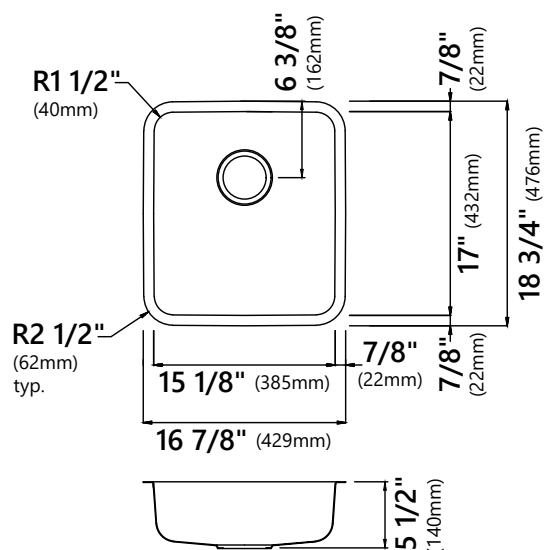
KA1AS17B 16\ 7/8'' \times 18\ 3/4'' \times 5\ 1/2'' Min Cabinet Size: 21"
