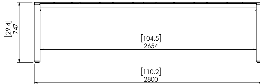
FRONT VIEW
