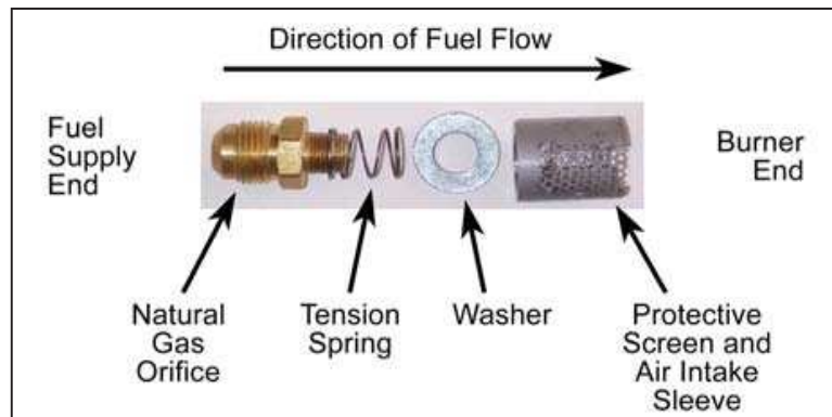
Orifice assembly for fire pit burners
