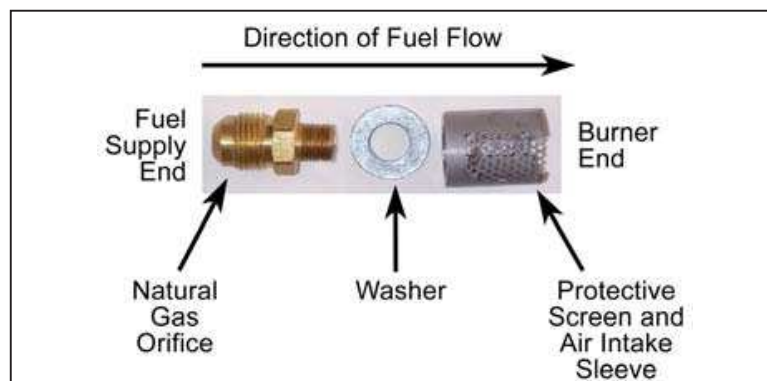
Orifice assembly for fireplace burners
