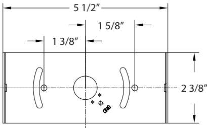
Back Plate Dimensions
