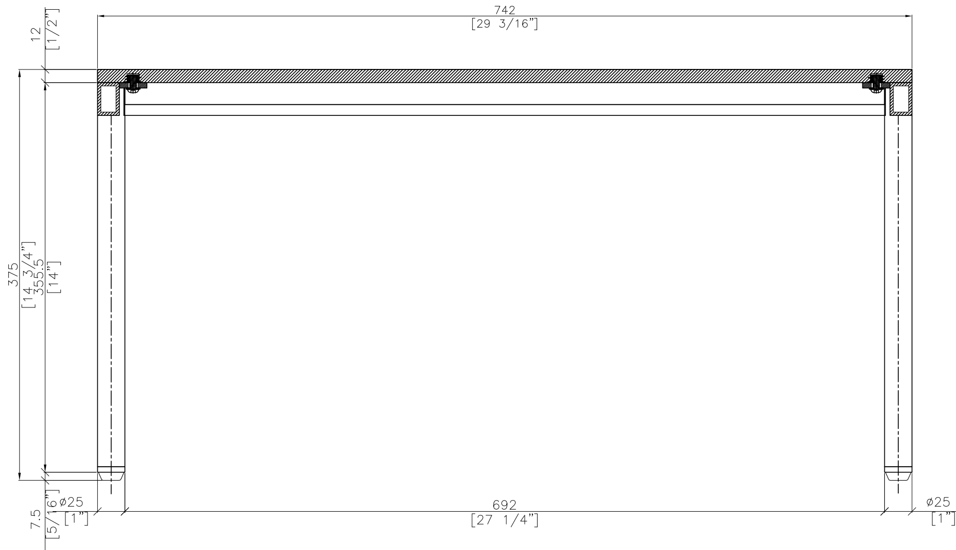
FRONT VIEW
