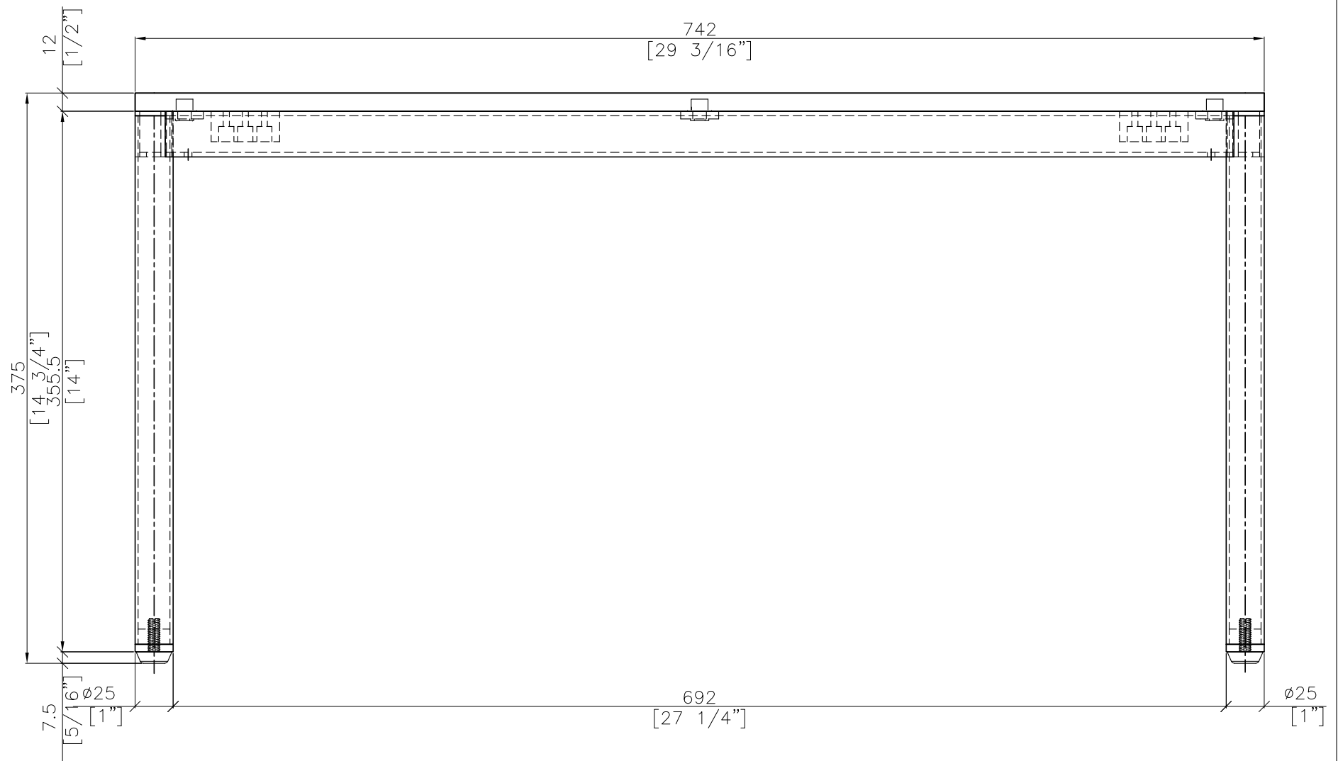
SIDE VIEW
