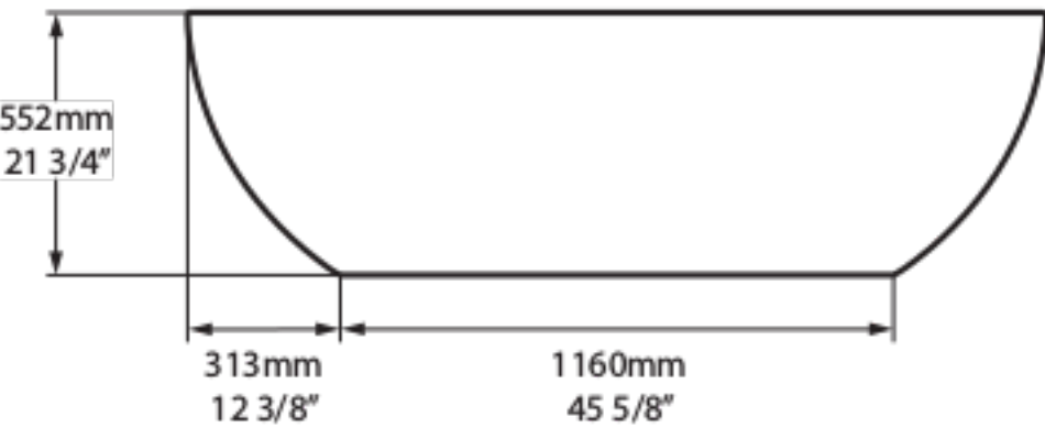
Side View
