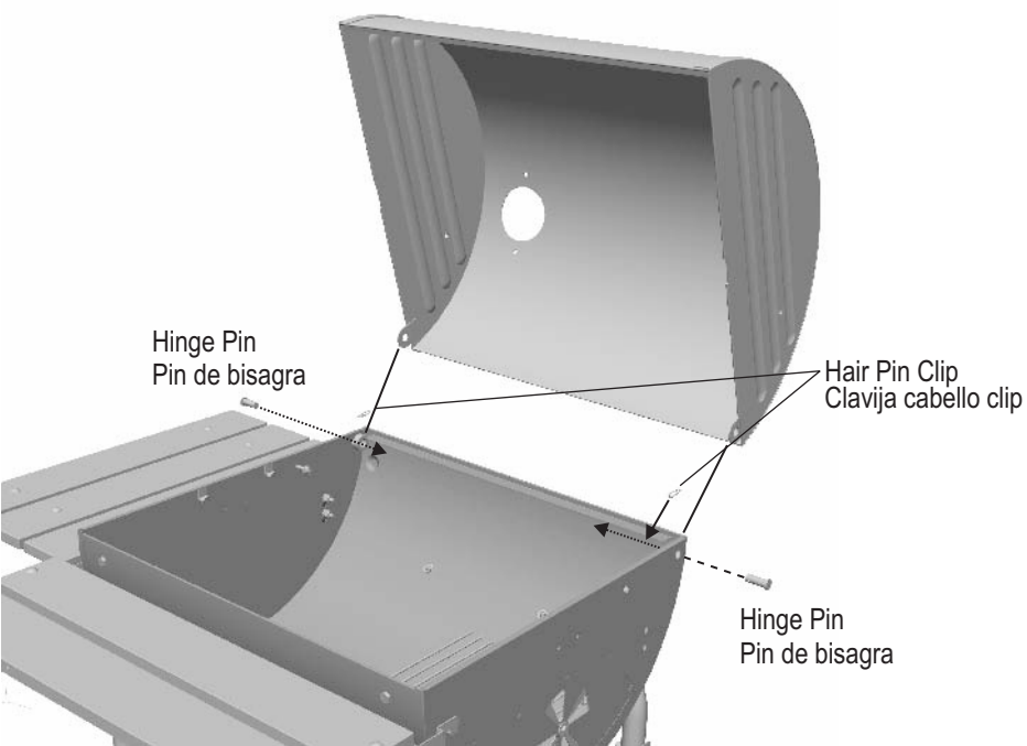
Hinge Properly Installed Bisagra correctamente instalado
