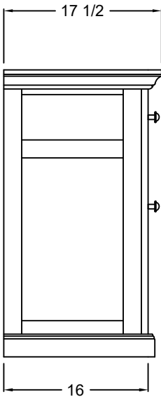
SIDE ELEVATION
