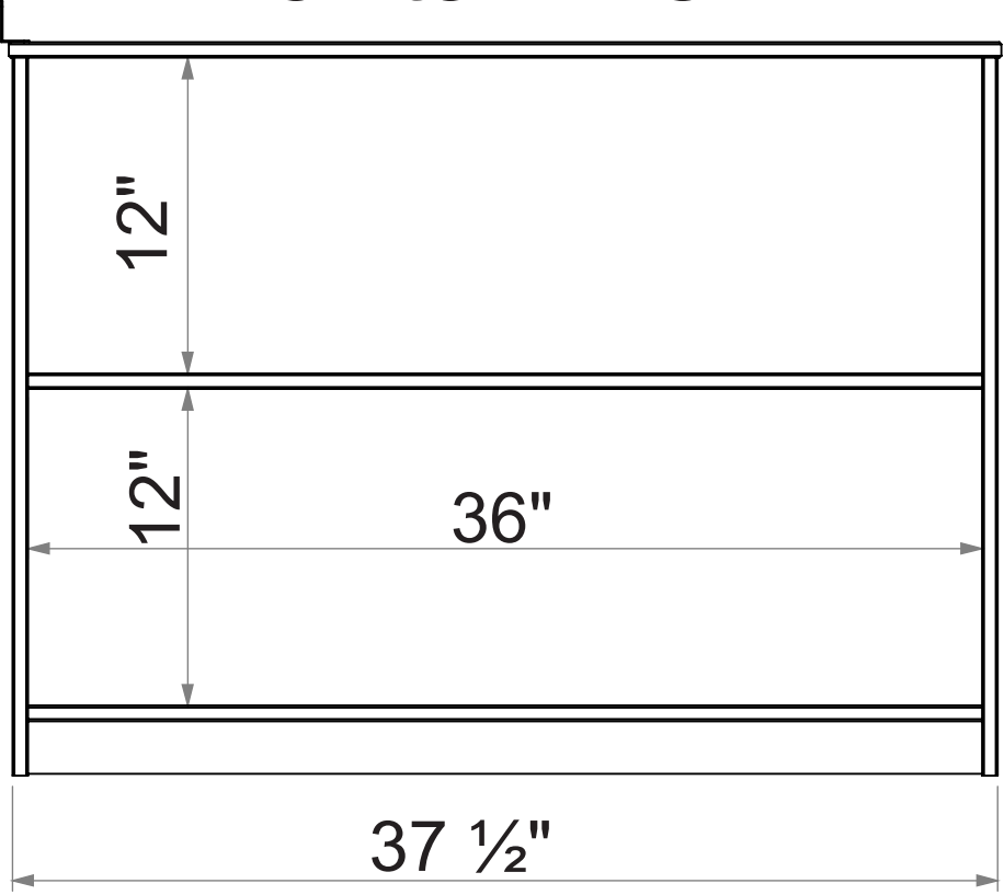
Frontal View
