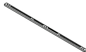
⑥ Center Rail 1905x50x35mm x 1pc
