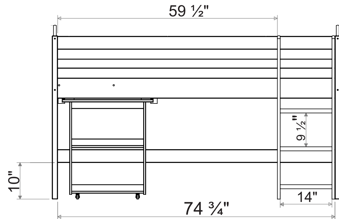
Frontal View
