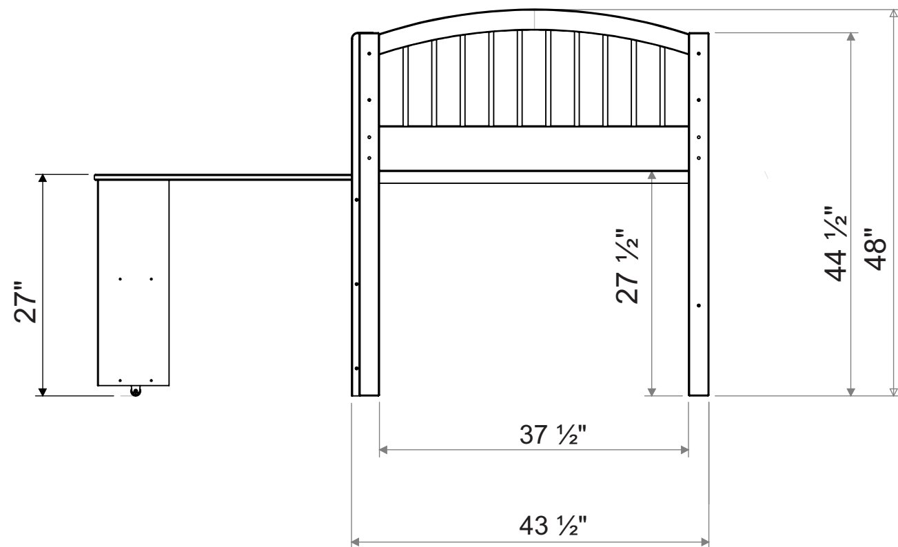
Loft Side View
