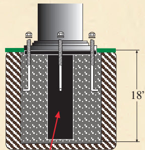
Direct Burial Kit
