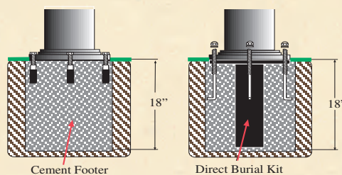
Posts can be Surface Mounted or installed as a Direct Burials
