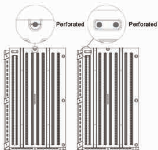
2OF3 Left Back Panel (1) GS0201002
