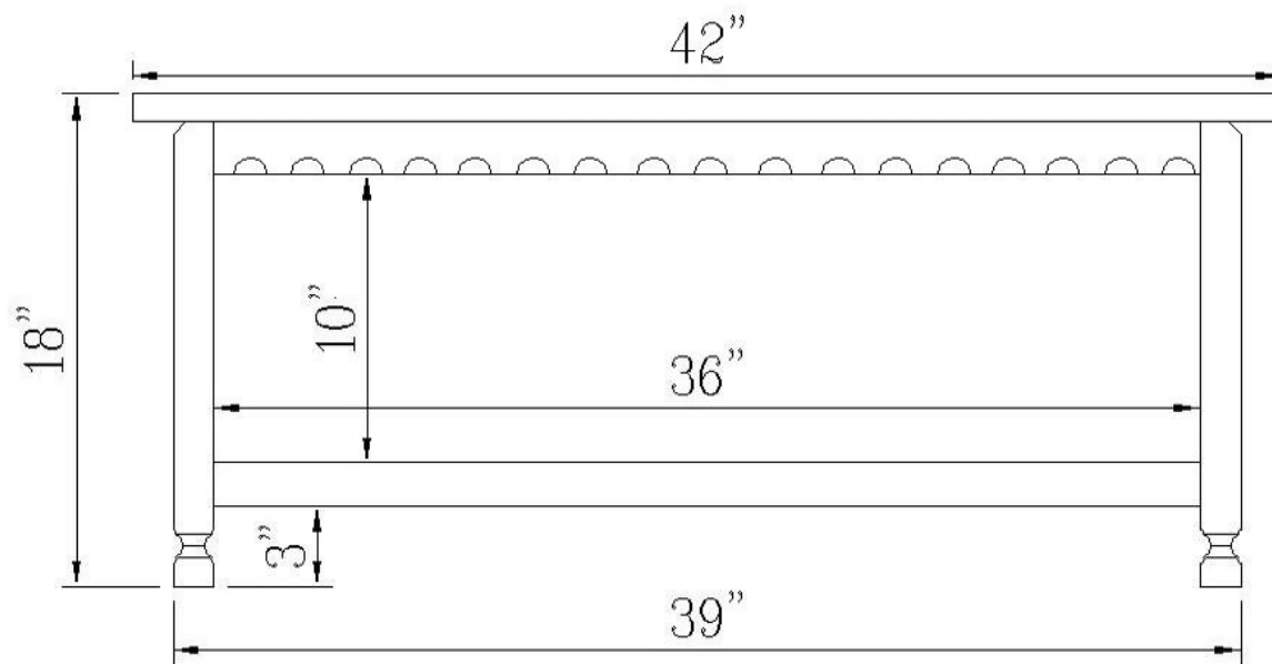
FRONT VIEW
