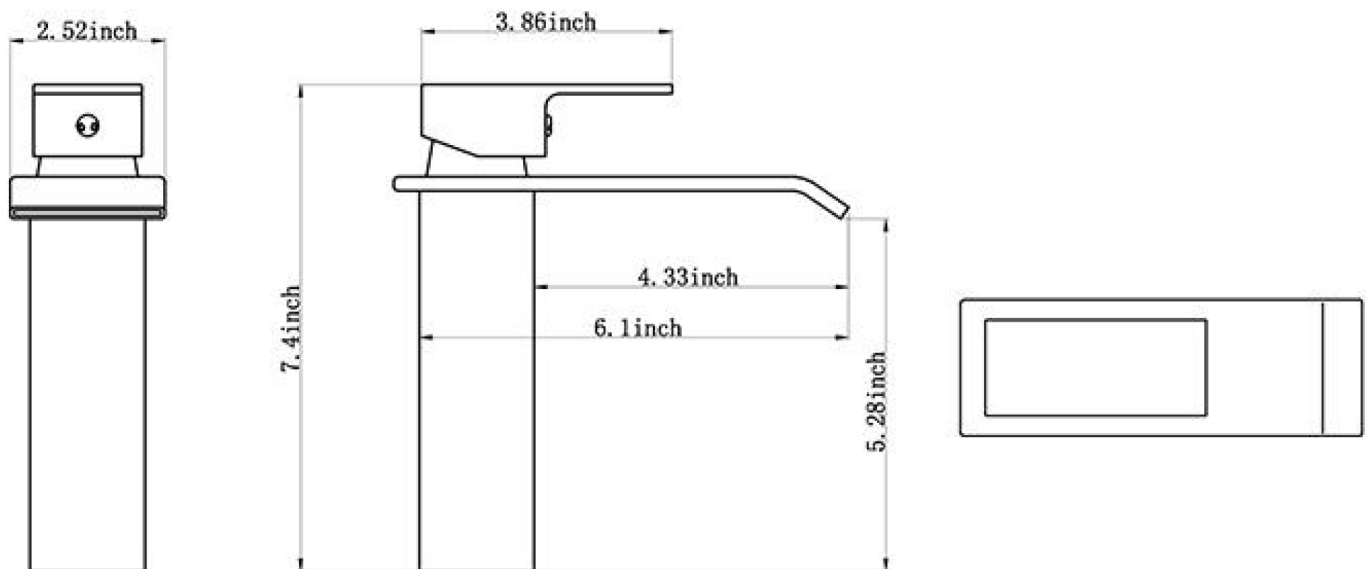
CRITICAL DIMENSIONS
