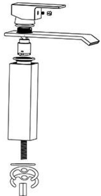
Single-Handle Lavatory Faucet
