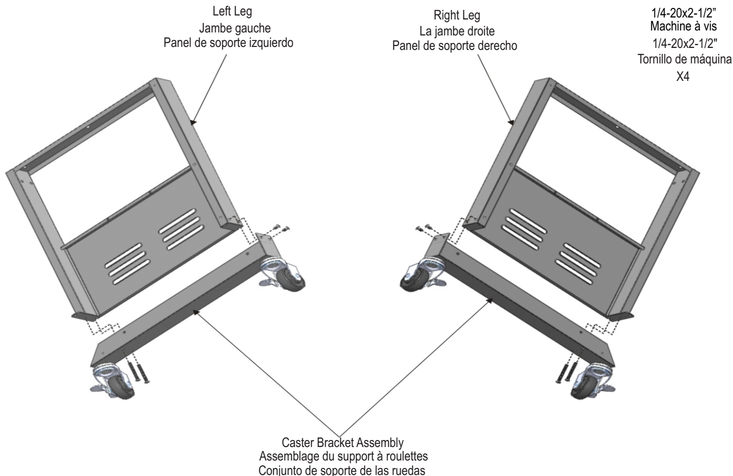
1/4-20x2-1/2" Machine screw
