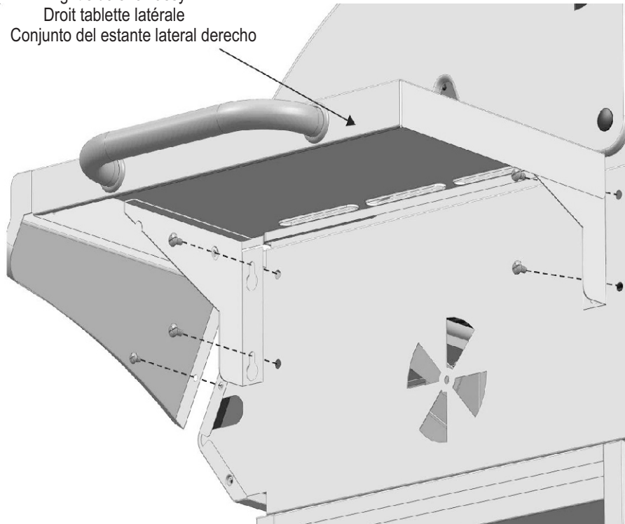
#10x3/8" Self-tap screw #10x3/8" Auto-bouchon à vis #10X3/8" Tornillo autorroscante X1
