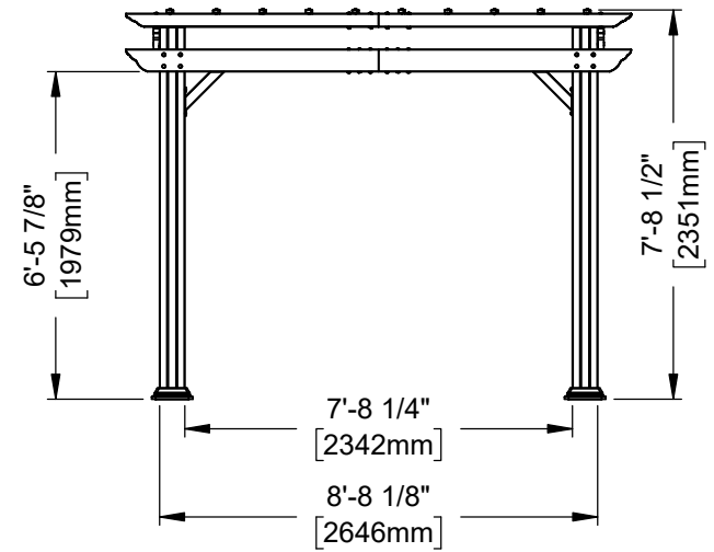
12' X 10' METAL PERGOLA FOOTPRINT
