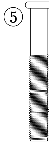
④ BOLT 1/4" X 1 3/4" x 3
