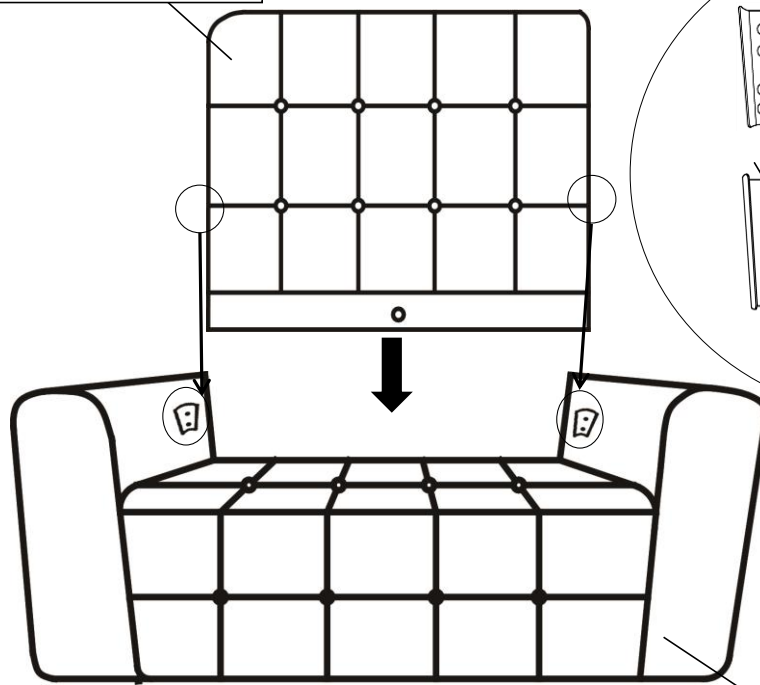
Chair Backrest(A)
