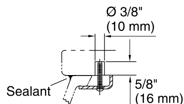
Marble Installation
