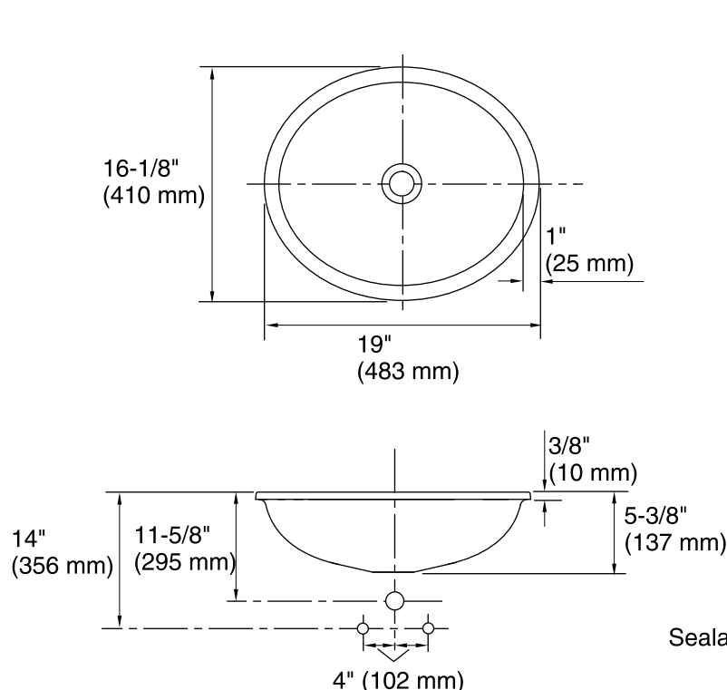
Standard Installation
