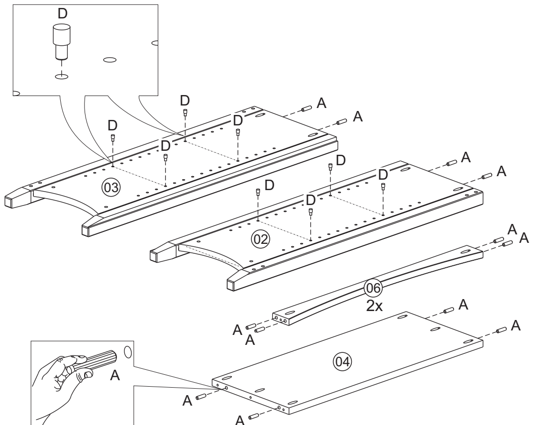
A - 8,0x30 Wood Dowel Qty. 16
