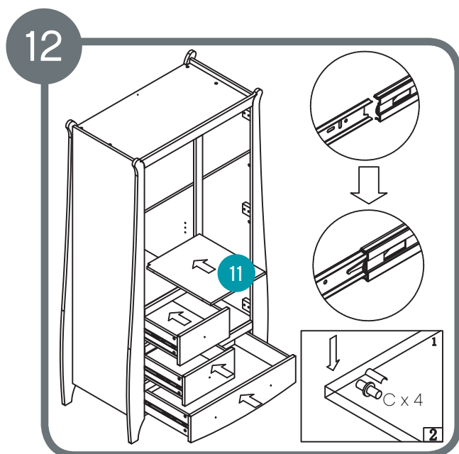
Assemble shelf and drawers.
