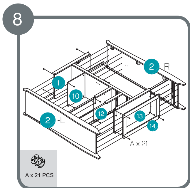
Assemble locking nuts 21 x A.
