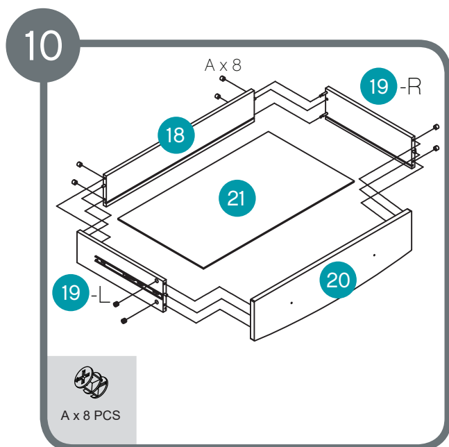
Assemble locking nuts 8 x A.
