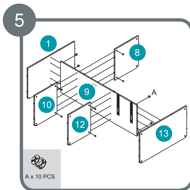
Assemble locking nut 10 x A.
