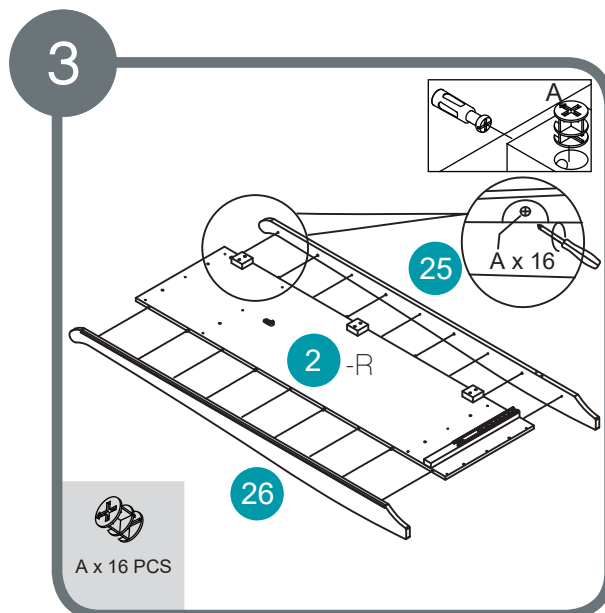
Assemble locking nut 16 x A.
