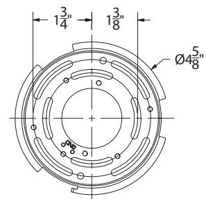
Mounting Backplate Dimensions
