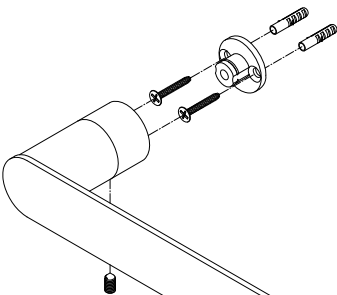
18" Towel Bar
