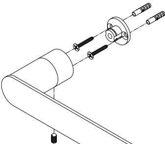
24" Towel Bar
