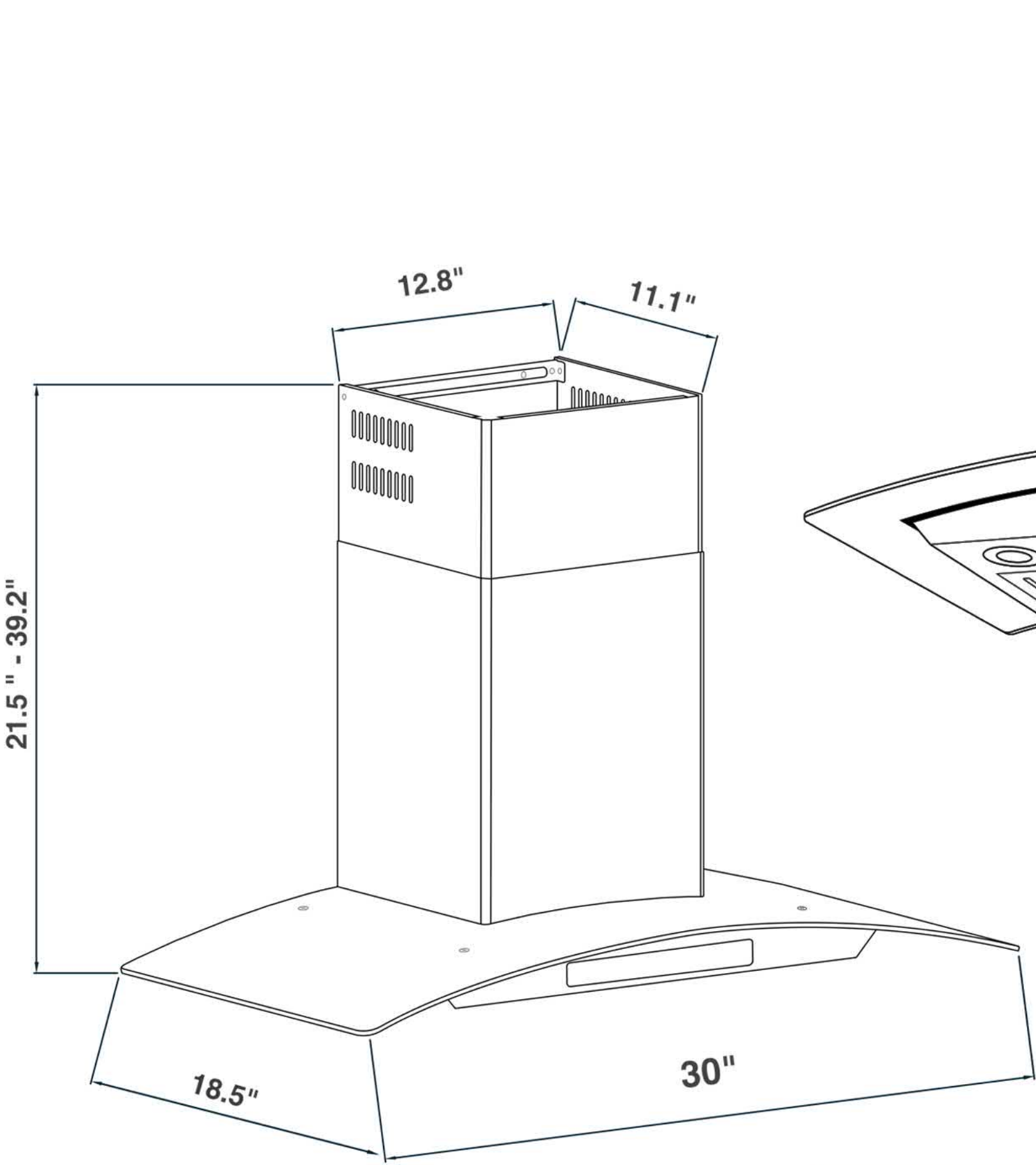
FRONT VIEW
