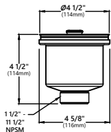
Model #: BST-1 Dimensions: \text{Ø}4 \frac{1}{2}" \times 4 \frac{1}{2}"
