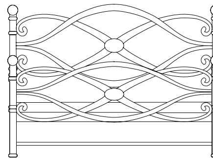
Low Post Bed, 5/0 Queen 66 1/8W x 90D x 59 1/2H (168 x 229 x 151 cm) Consists of: 5/0 Low Post Headboard 66 1/8W x 4D x 59 1/2H (168 x 10 x 151 cm) 5/0 Low Post Footboard 66 1/8W x 4D x 40H (168 x 10 x 102 cm) 5/0 Low Post Rails w/CSS 82W x 1 3/4D x 6 1/2H (208 x 4 x 17 cm)
