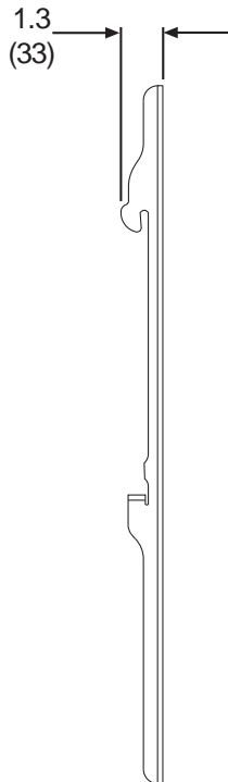
Shallow Adapter Bracket Detail
