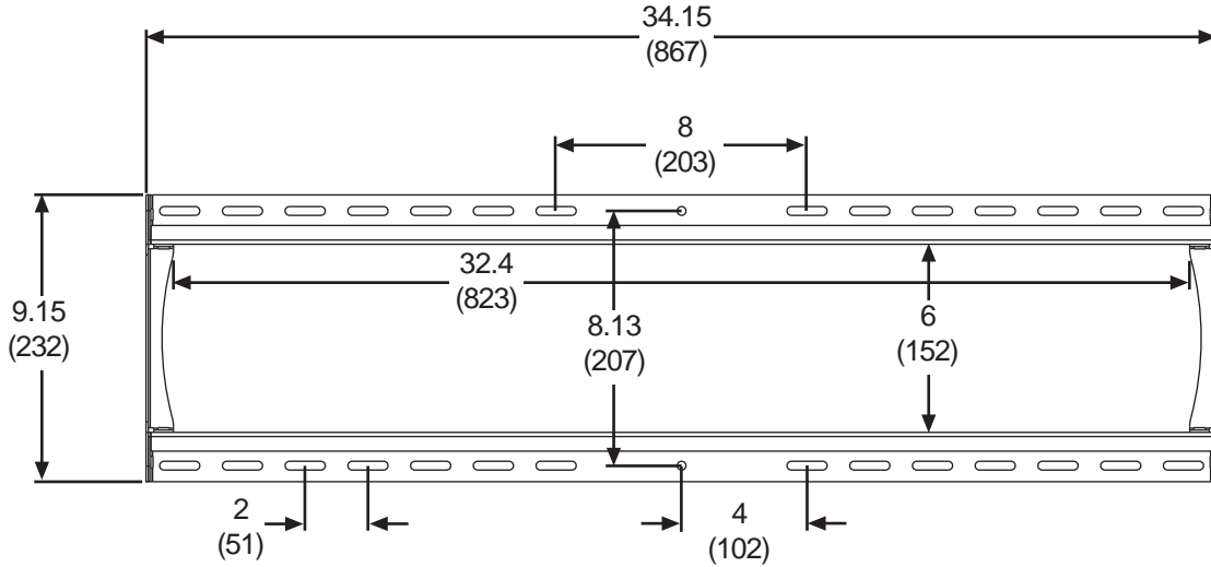
Wall Plate Detail
