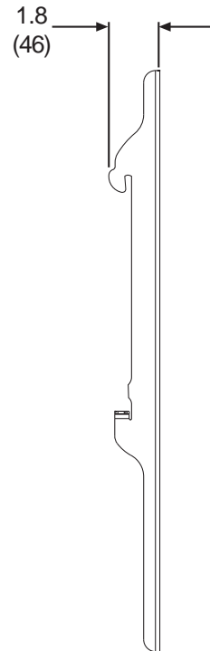
Deep Adapter Bracket Detail
